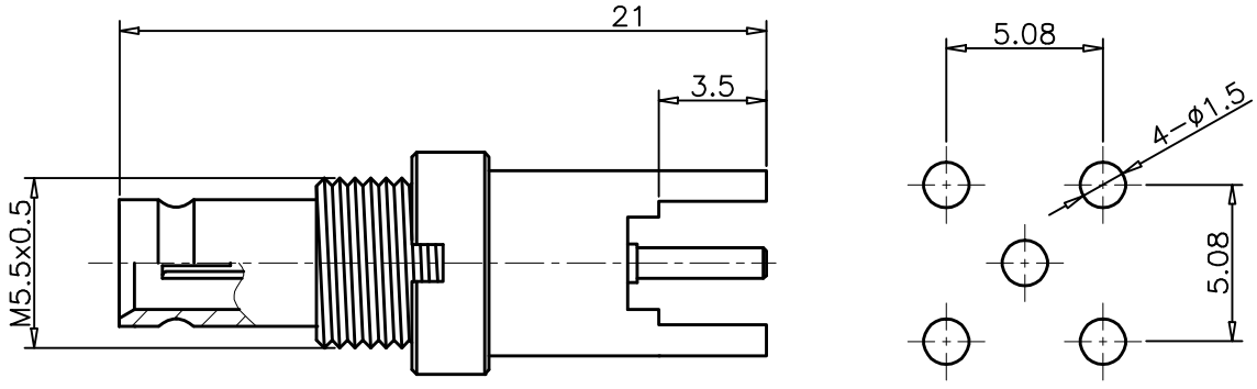
mounting detail
